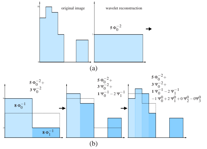
Fig. 3 The 1D image (upper, left) is: [8, 10, 9, 5, 0, 0, 4, 4] , and its unnormalized (used here because it is simpler to display) Haar representation is: [5, 3, 1, -2, 0, 0] . The image is then reconstructed one level at a time as follows: [5] \rightarrow [5 + 3, 5 - 3] = [8, 2] \rightarrow [8 + 1, 8 - 1, 2 - 2, 2 + 2] = [9, 7, 0, 4] and so on. Here 0 is the finest scale index or the scale where data is gathered and -2 is the coarsest scale.
