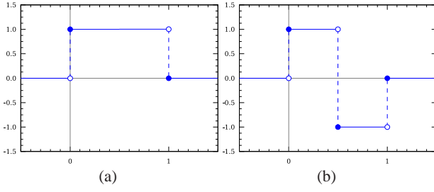
Fig. 2 1D Haar mother functions, left the scale mother function \Phi and right the scale wavelet function \Psi .
